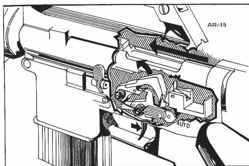
AR-15 WITH DROP-IN AUTO-SEAR
